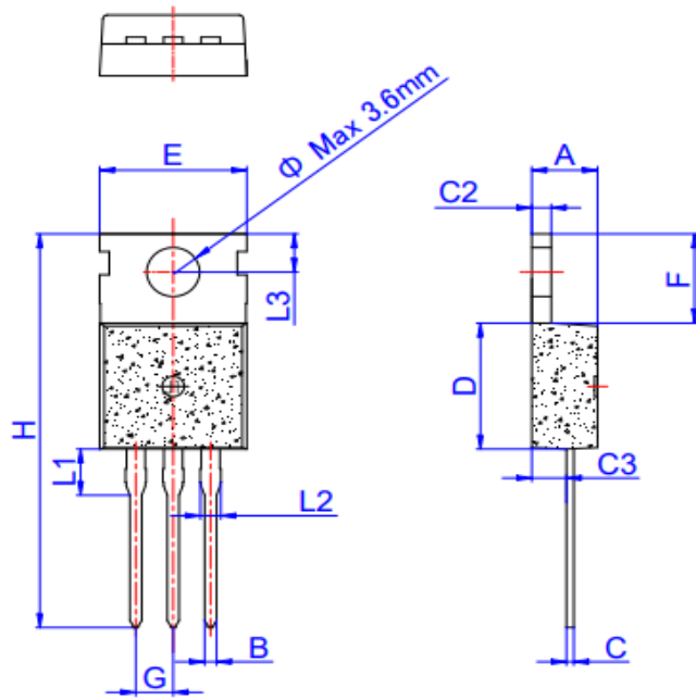
TO-220C
